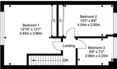
Second Floor Approximate Floor Area 442.82 SQ.FT. (41.14 SQ.M.)
